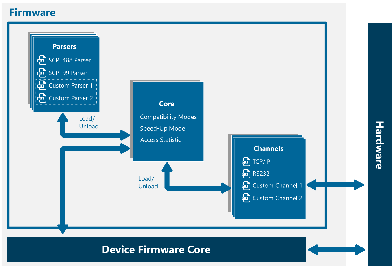
Fig. 1: Poseidon communicates with the Firmware and the hardware of the device.
